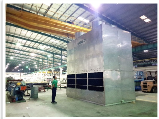
Manufacturing: SS304 Condenser Zone
